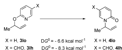
Scheme 6. DFT calculation on the stability for O - and N -allylated 2-pyridones in the gas phase.
