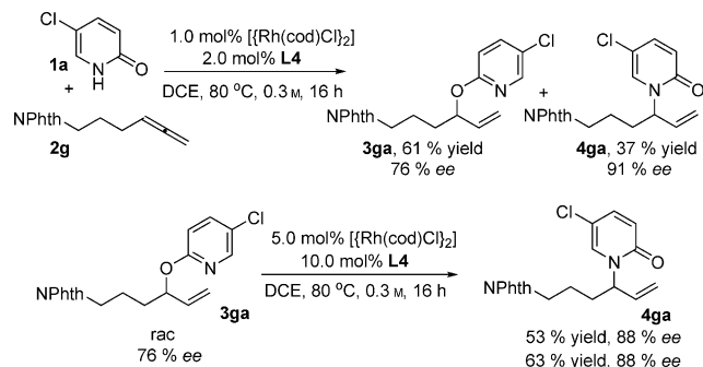
Scheme 5. Conversion of O -allylated product into N -allylated product.
