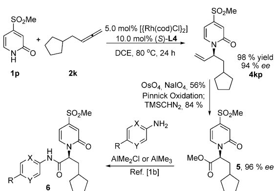
Scheme 8. The synthesis of glucokinase activators 6 .
