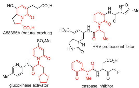
Figure 1. Biologically active molecules with N -chiral 2-pyridone moieties.
