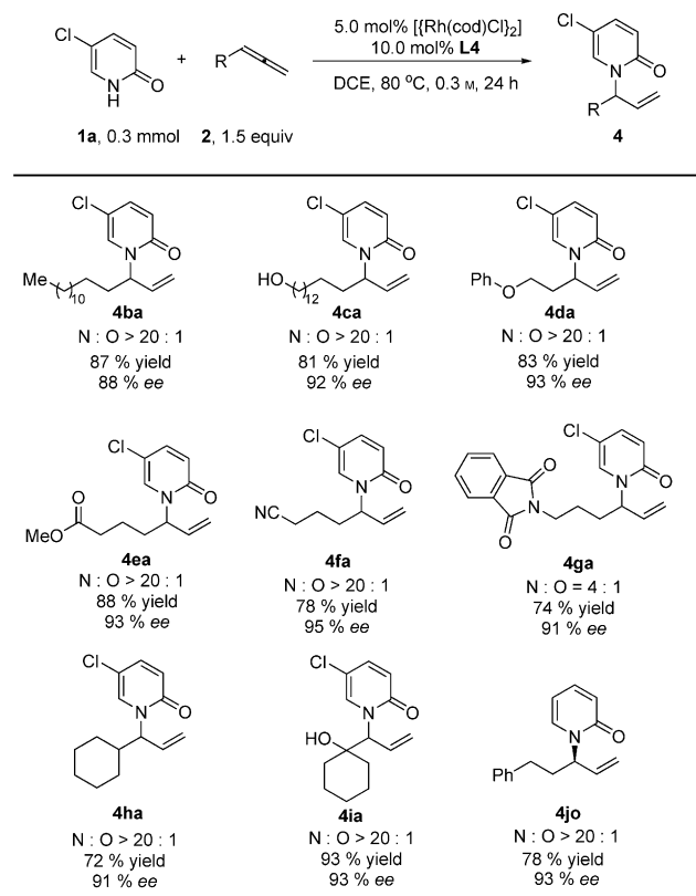
Scheme 4. Scope of allenes in the rhodium-catalyzed chemo-, regio-, and enantioselective addition of 2-pyridones to allenes.
