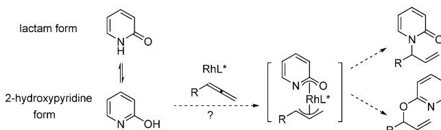
Scheme 2. The rhodium catalyst differentiates two tautomers and determines the O vs. N ratio.
