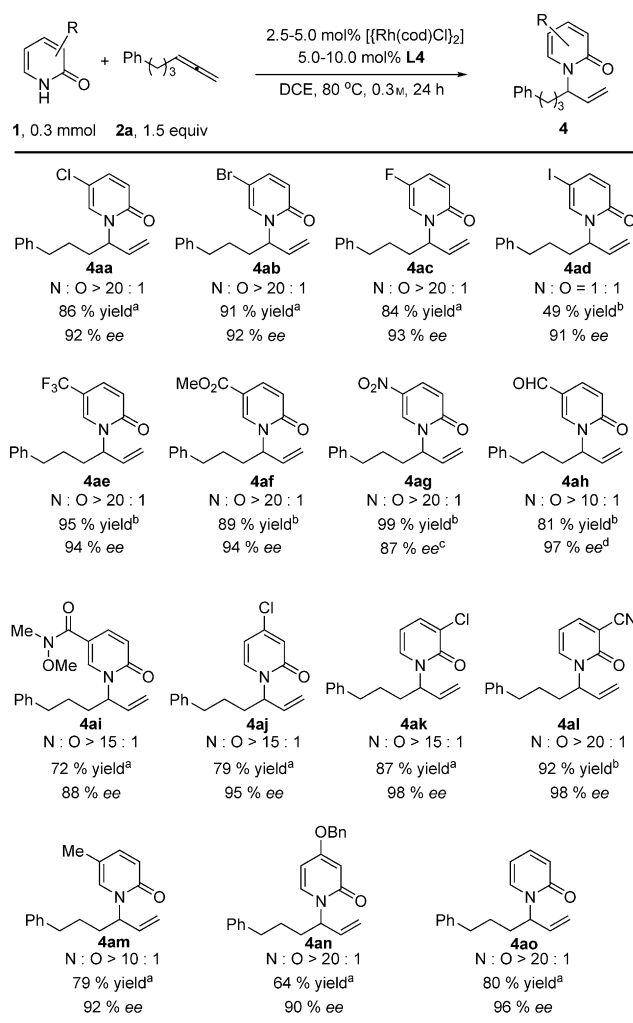
Scheme 3. Scope of 2-pyridones in the rhodium-catalyzed chemo-, regio-, and enantioselective addition of 2-pyridones to allenes.
